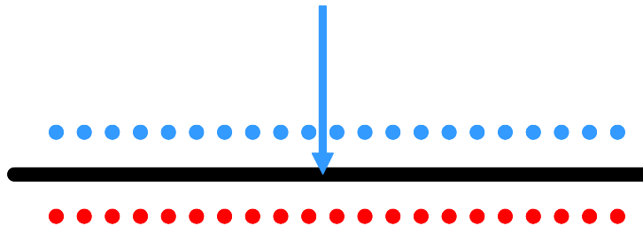
Figure 4. Conditions to use the Pressure on both sides option. The top surface pressure (blue arrow) will be calculated using the pressure points above the element surface (blue dots), and the pressure on the bottom surface will be calculated using the pressure points below the element surface (red dots). The net pressure will be calculated by subtracting the bottom pressure from the top pressure.
