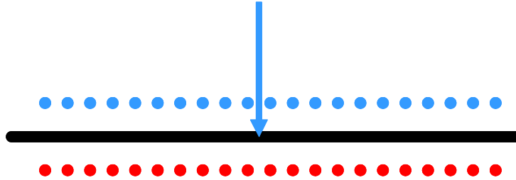
Figure 3. Conditions to use the Pressure on one side – directional dependent option. The pressure is applied to the top surface (blue arrow), and the pressure points above the element surface (blue dots) will be used in the pressure calculation. The pressure points on the below the element surface (red dots) will be ignored.
