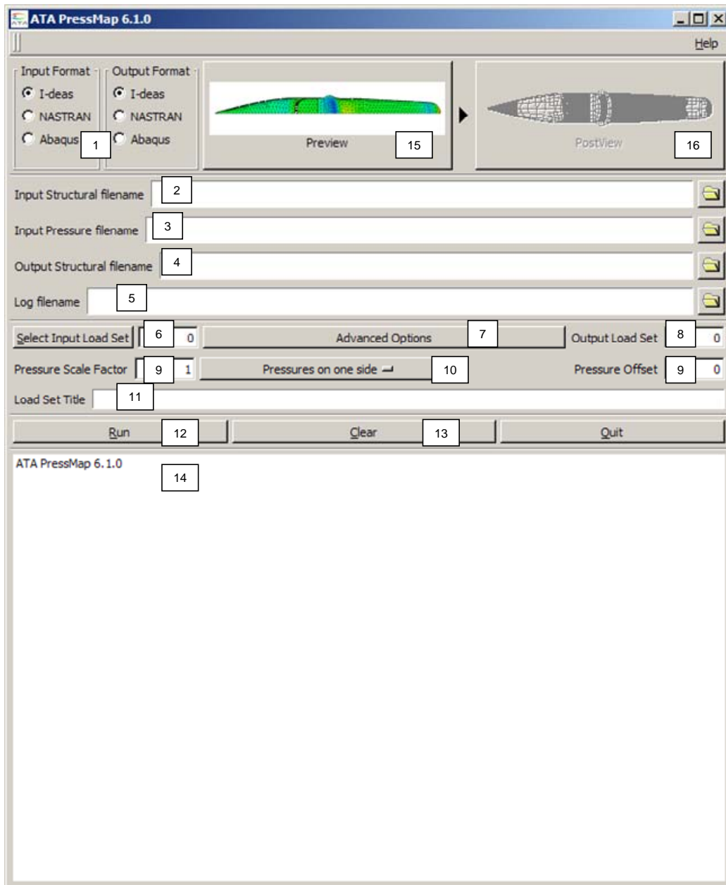
Figure 1. PressMap interface showing the key input and output fields.
