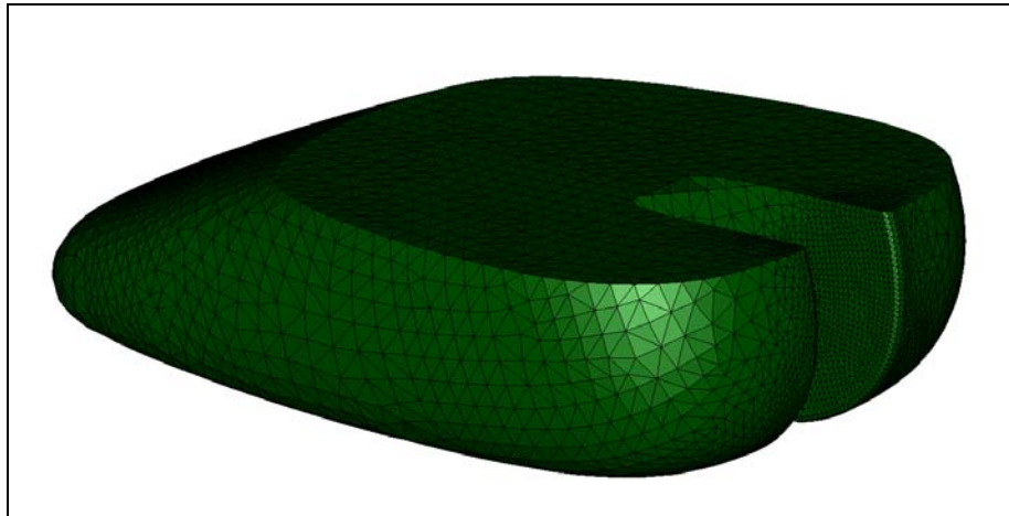
Figure 4-30. Fluid surface elements (wetted tank and free surface).
