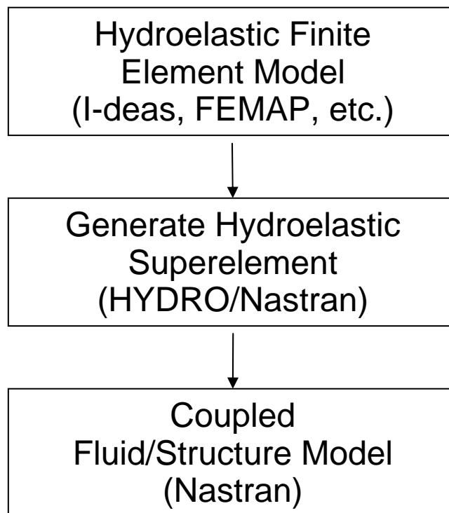
Figure 1-2. A hydroelastic model is developed in a three-step process.
