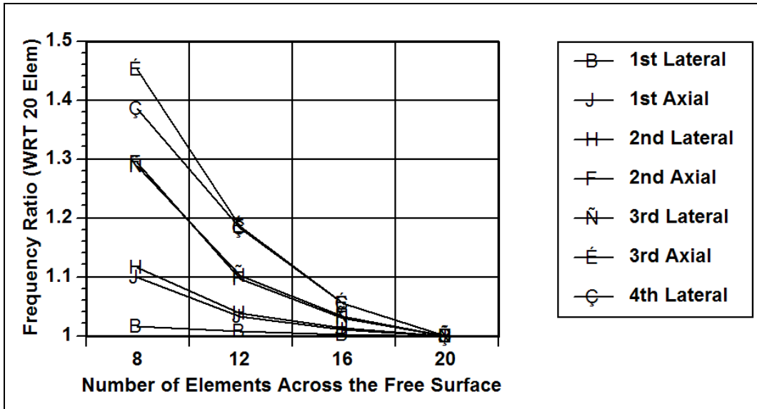
Figure 5-2. At least sixteen elements across the free surface were required to obtain 5% accuracy on the third lateral slosh mode for the Titan IV Centaur modal survey test configuration.
