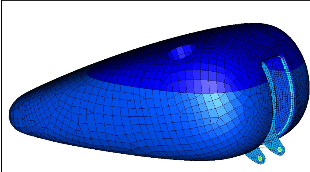
Figure 4-28. Outer shell of motorcycle tank example.
