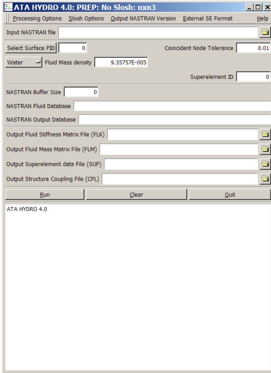
Figure 4-13. HYDRO GUI input for fluid hemisphere example with NO_SLOSH_STD option.
