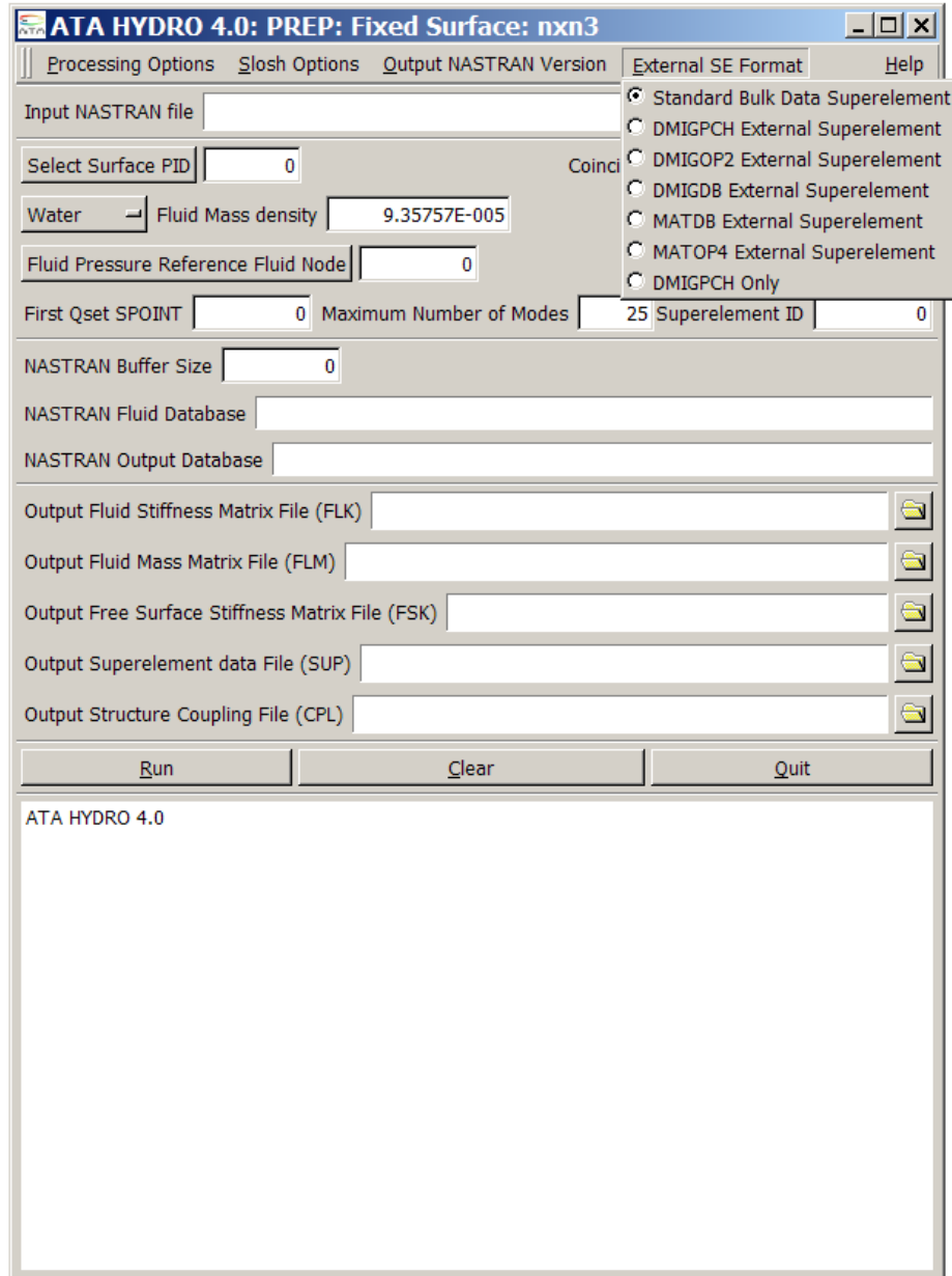
Figure 5-6. External superelement options.
