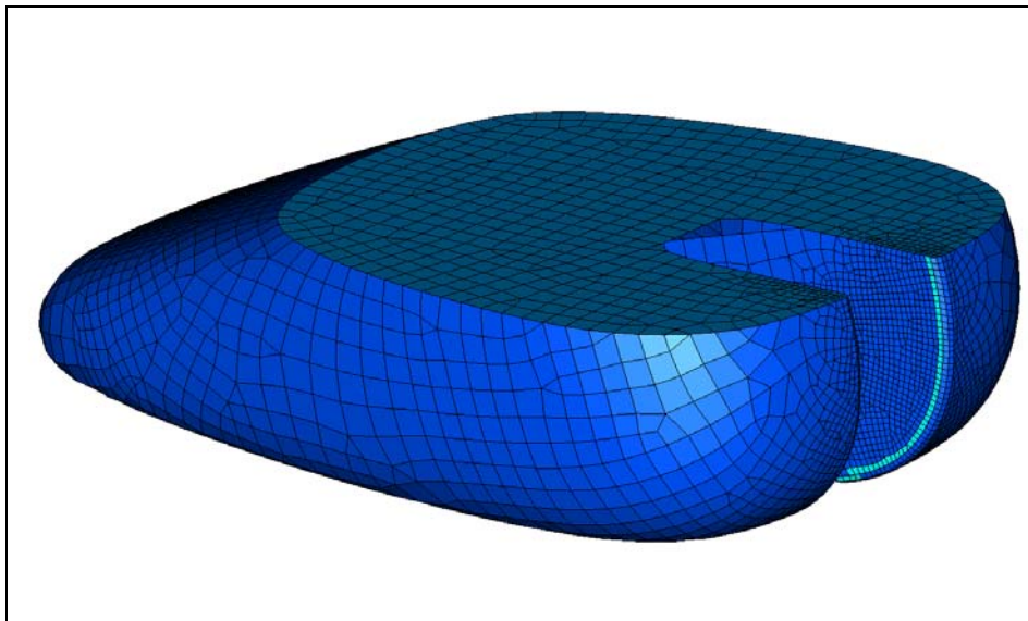
Figure 4-29. Fluid surface elements (wetted tank and free surface).
