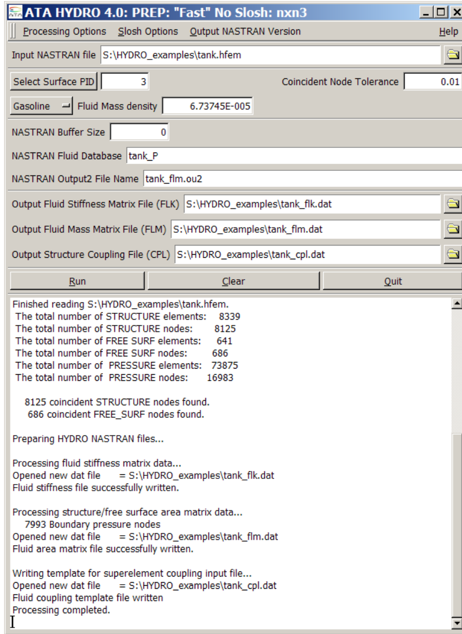
Figure 4-32. HYDRO GUI input for fluid hemisphere example with ENCLOSED option.
