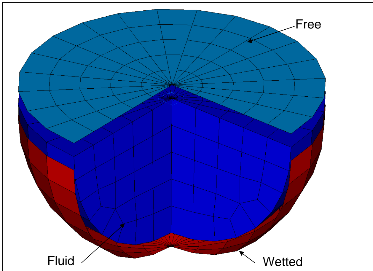
Figure 3-3. The hydroelastic finite element model will include solid elements for the fluid and shell elements for the wetted structure and free surface (exploded view).
