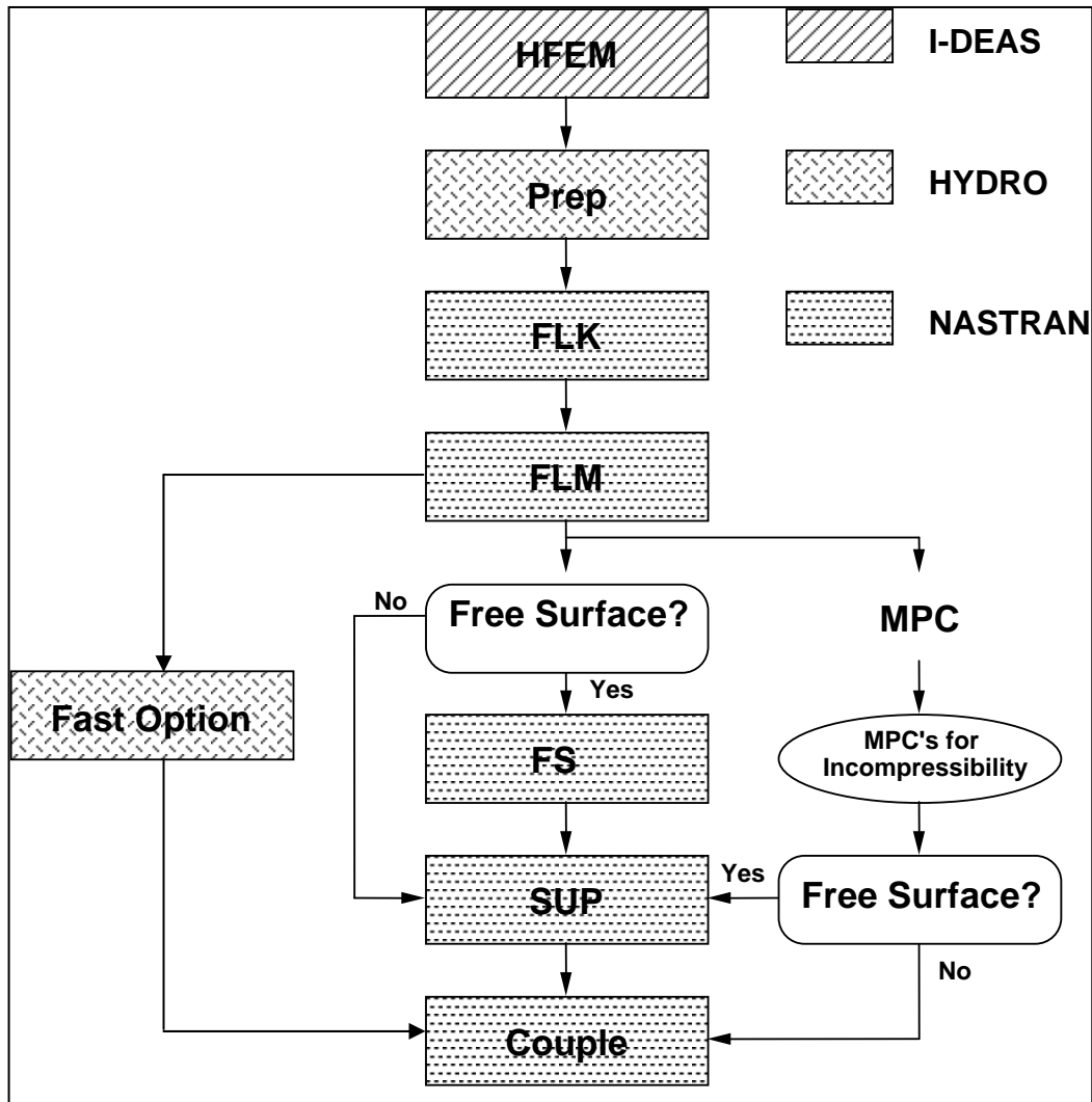
Figure 3-1. The coupled hydroelastic model is formed using NASTRAN and a special Fortran program called HYDRO.
