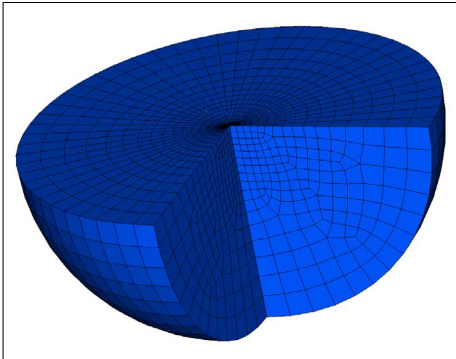
Figure 5-3. Fine mesh representation of hemisphere example problem.
