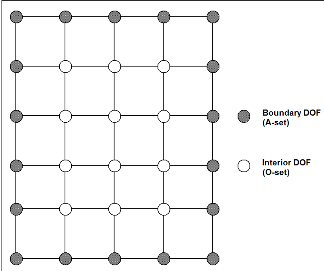
Figure 2-2. The finite element model of an incompressible fluid can be mathematically reduced to the boundary nodes with no loss of accuracy.
