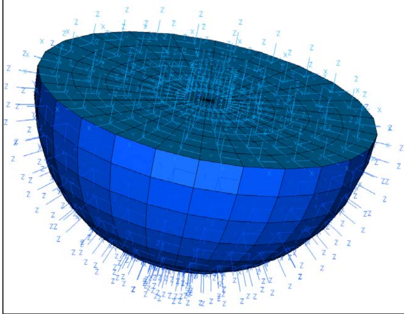
Figure 4-4. The orientation of the wetted structure and free surface shells were checked to verify that their orientation was uniformly outward.
