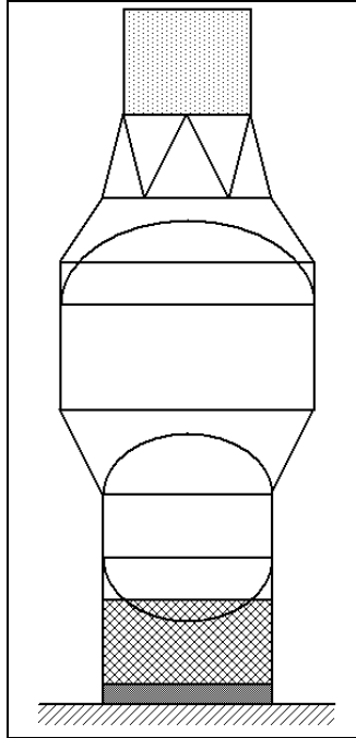
Figure 5-1. Titan/Centaur modal survey configuration.
