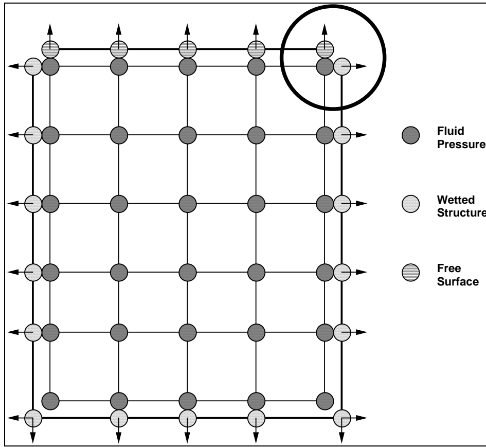
Figure 3-2. There will be three coincident nodes at the intersection of the fluid, wetted-structure and free surface.
