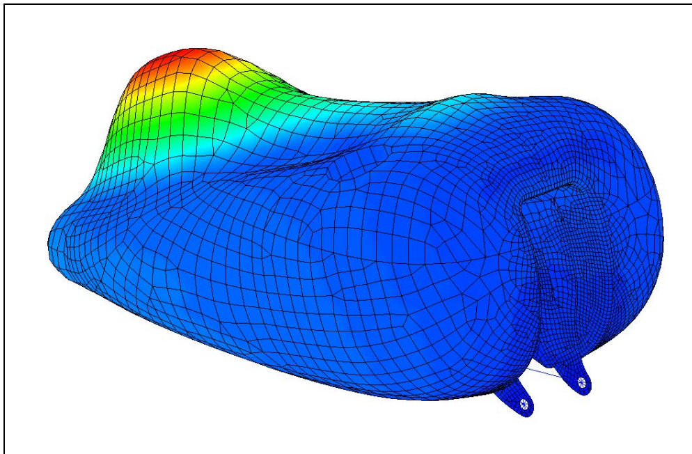
Figure 4-39. First flexible coupled mode for motorcycle tank.
