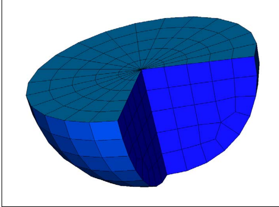
Figure 2-1. Fluid is modeled with linear solid elements.
