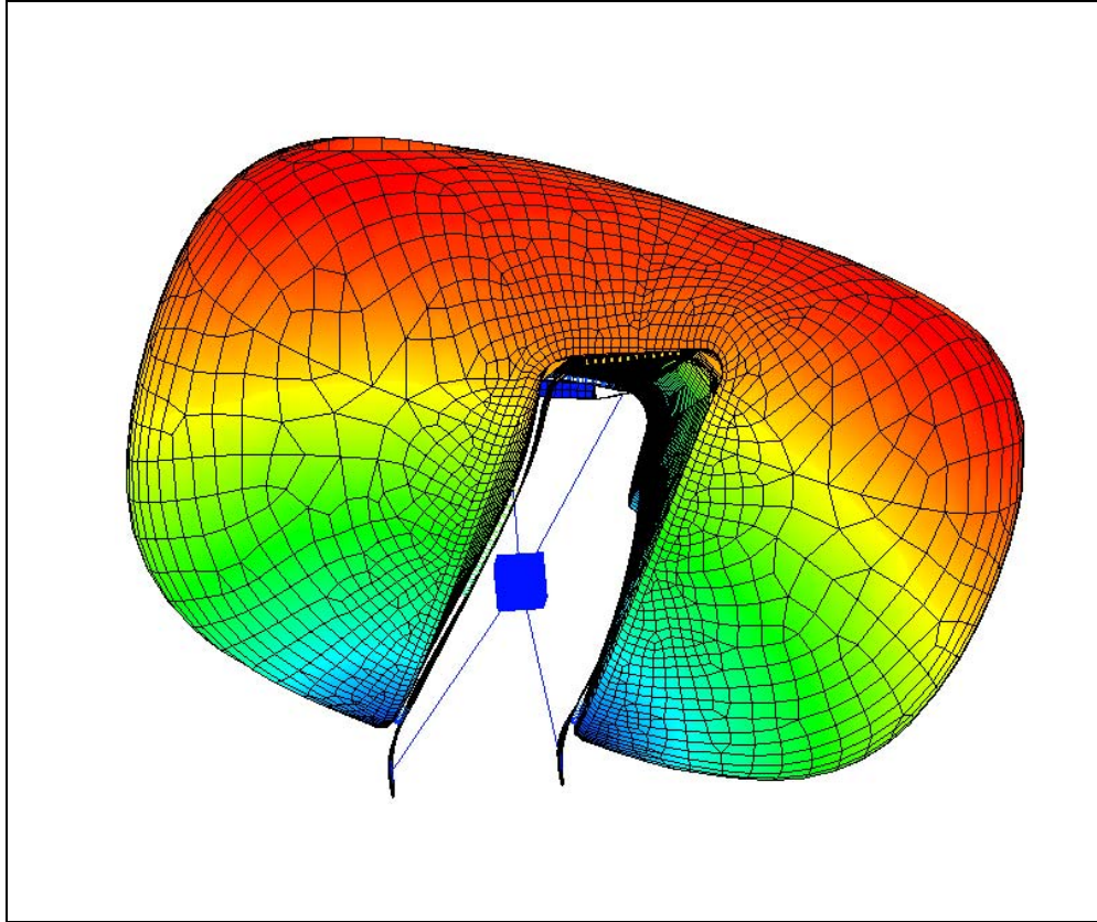
Figure 4-38. First flexible coupled mode for motorcycle tank.
