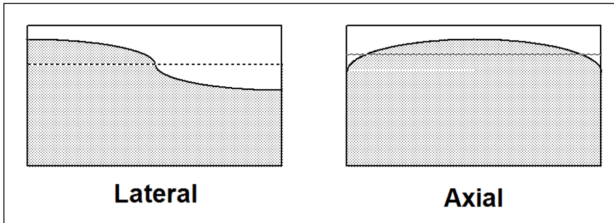
Figure 2-4. Lateral and axial slosh modes occur when the fluid has a free surface and is in a gravity field.
