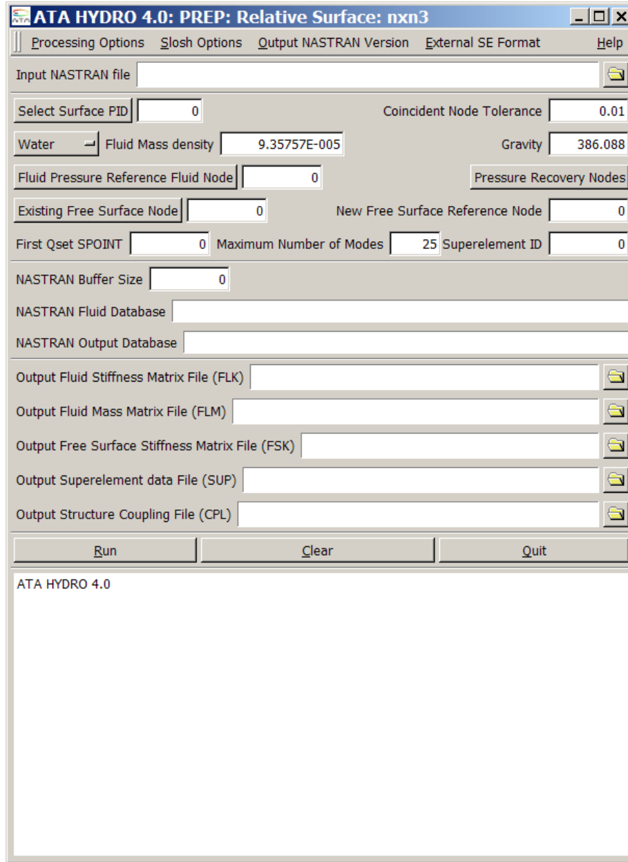
Figure 4-14. HYDRO GUI input for fluid hemisphere example with RELATIVE option.
