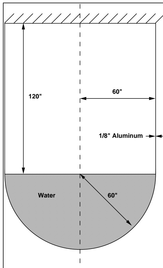
Figure 4-1. The example problem includes a hemisphere of water in a thin-walled tank.
