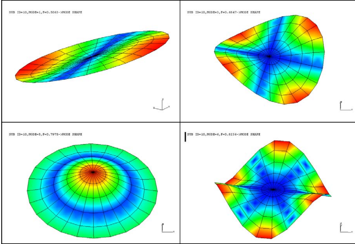
Figure 2-5. Large numbers of axial and lateral slosh modes will exist when the fluid has a free surface.
