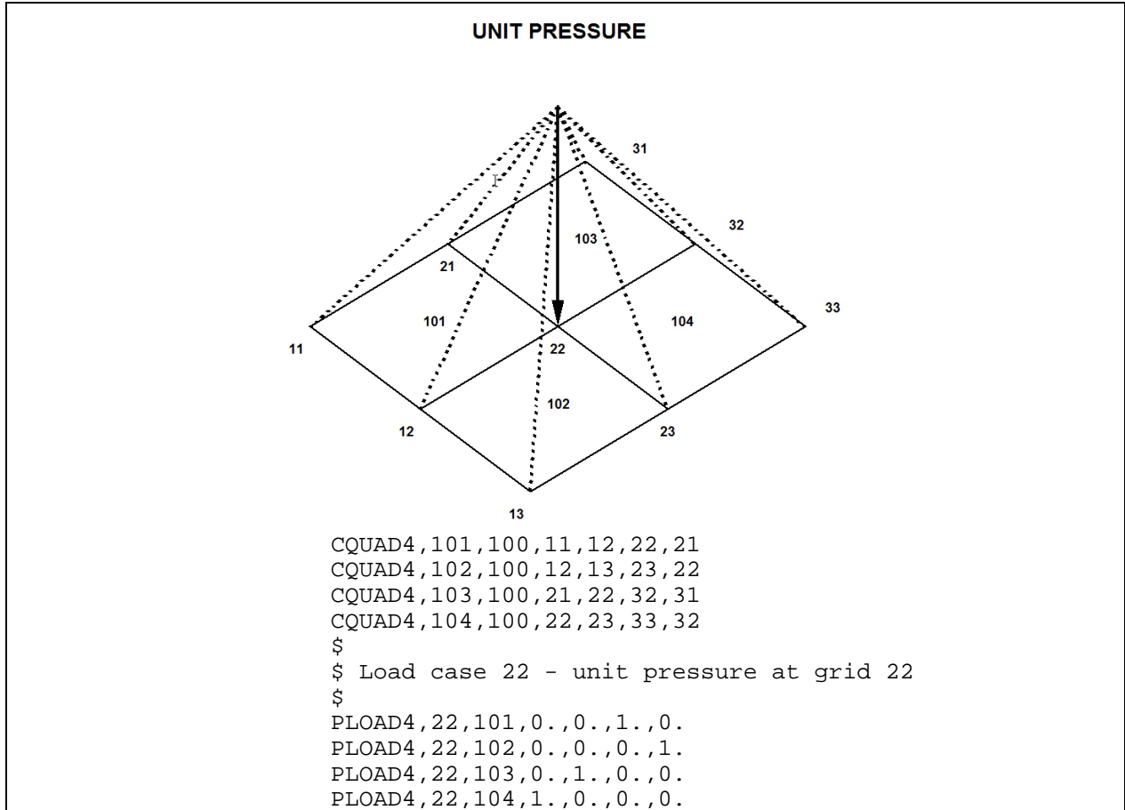
Figure 2-3. A column of the area matrix contains the structural forces caused by a unit pressure at a fluid boundary node.
