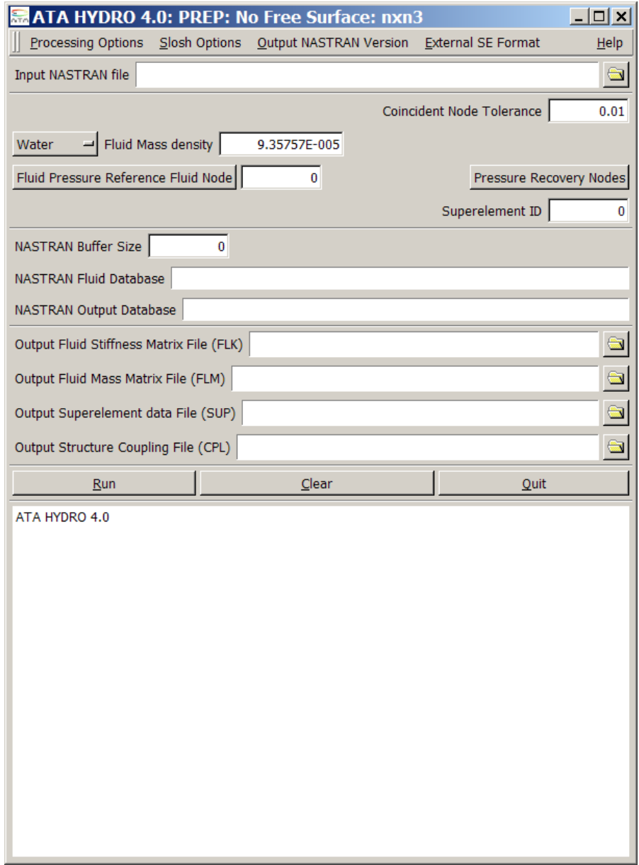
Figure 4-10. HYDRO GUI input for fluid hemisphere example with ENCLOSED option.
