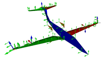
Measurement locations: Full aircraft
