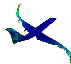
Example measured mode of vibration
