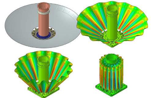
Select frames from the stowing simulation
