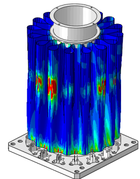
RMS stress from random analysis
