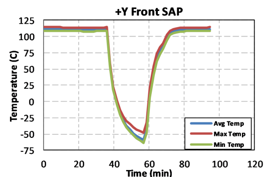
Maximum/Minimum temperatures of front side of +Y SAP as a function of time
