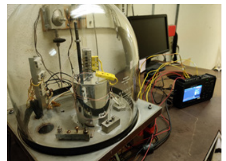
Hi-Z RPS in a thermal vacuum testing chamber
