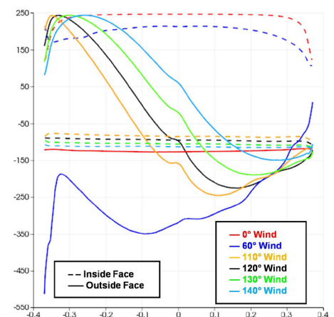
Dish centerline pressure profiles
